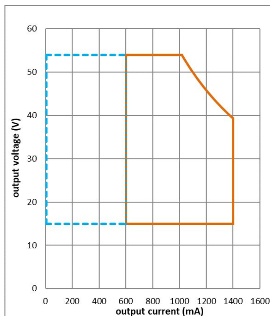
OTI DALI 50 NFC LP Operating window
